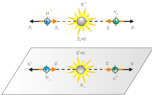
Parity-violating collinear decay of a pion \pi^+ at rest into a muon \mu^+ and a muonic neutrino \nu_\mu .
