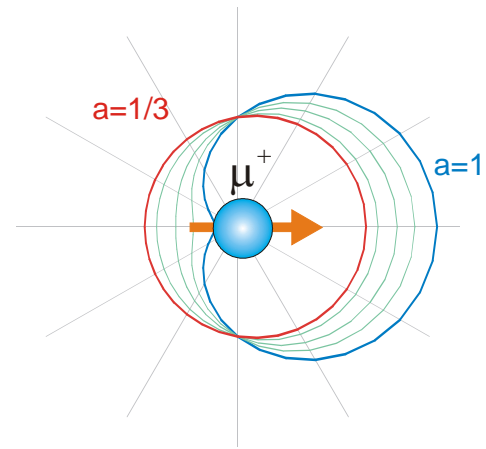
Angular distribution of the positrons from the muon decay: W(E,\theta) = 1 + a(E)\cos(\theta) . When all positron energies E are sampled with equal probability the asymmetry parameter has the value a = 1/3 (red curve).
